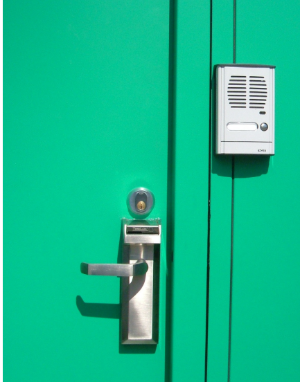
Assa Timelox access via card insertion. Intercom access request using electric strike.
